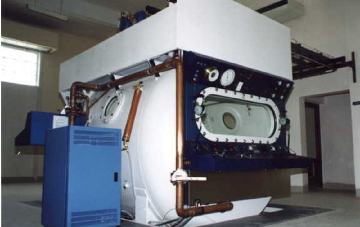
PCCI Model ATR-6 (cylindrical), Aviation Training Altitude Chamber, Dual Compartment, installed at Bangladesh Air Force base in Dhaka, Bangladesh
